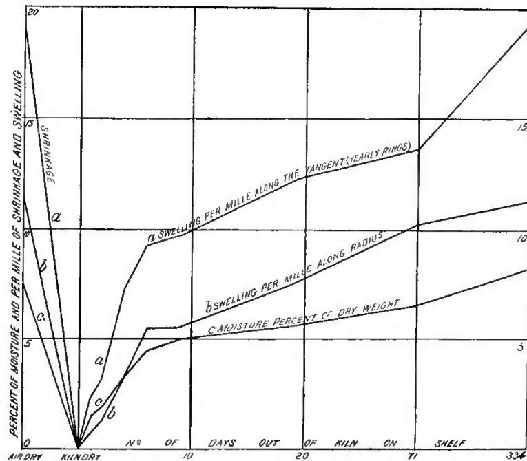
FIG. 4.—Diagram showing loss of water in kiln drying and reabsorption in air, shrinking and swelling.
